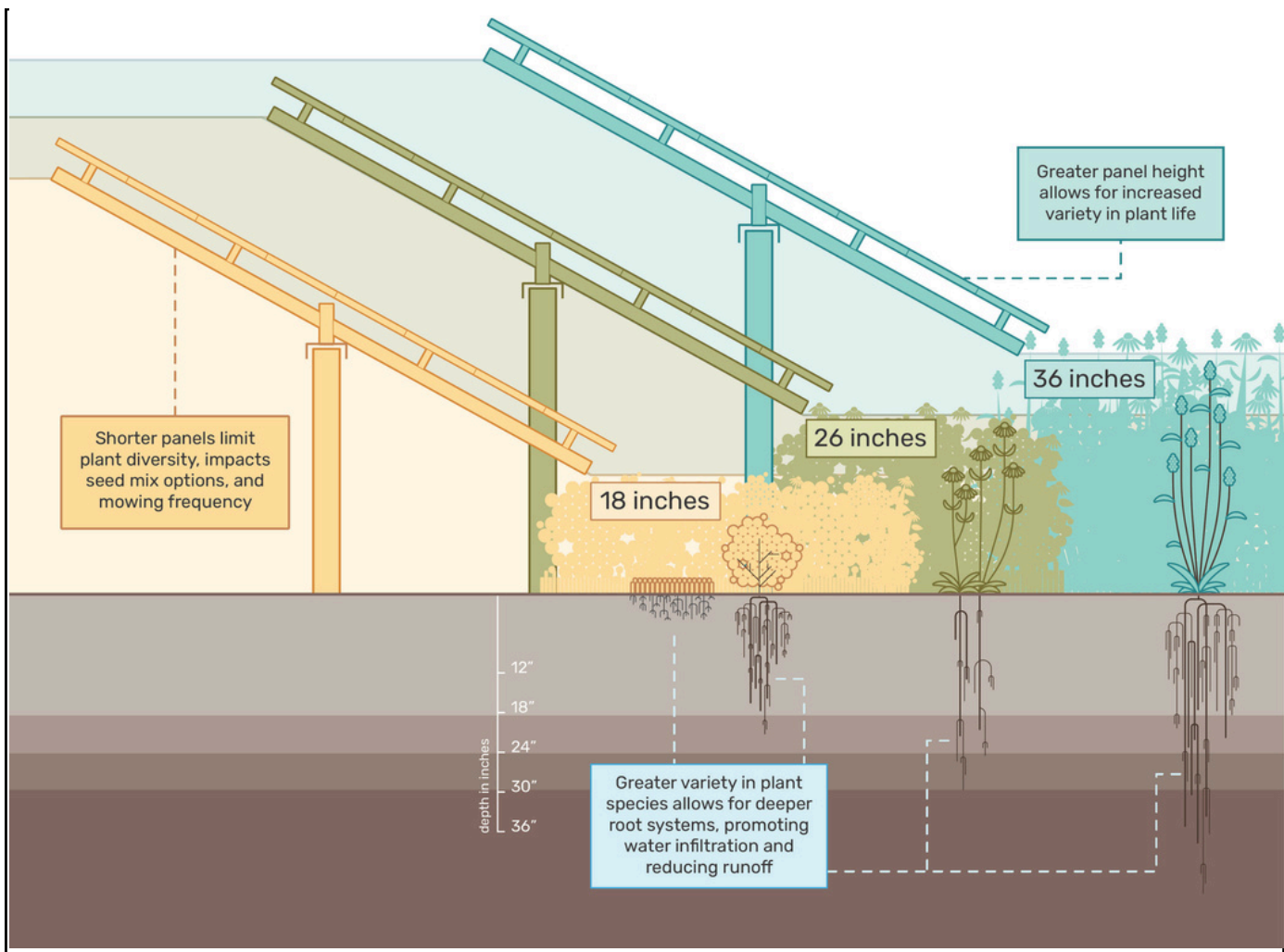
Figure 1. Solar panel height impact on vegetation. Illustration by Kay Rossback, reprinted from Ross et al., Best Practices: Photovoltaic Stormwater Management Research and Testing (PV-SMaRT) , 12. Increasing panel height allows for a wider range of deep-rooted vegetation to grow, slowing runoff and improving infiltration.
